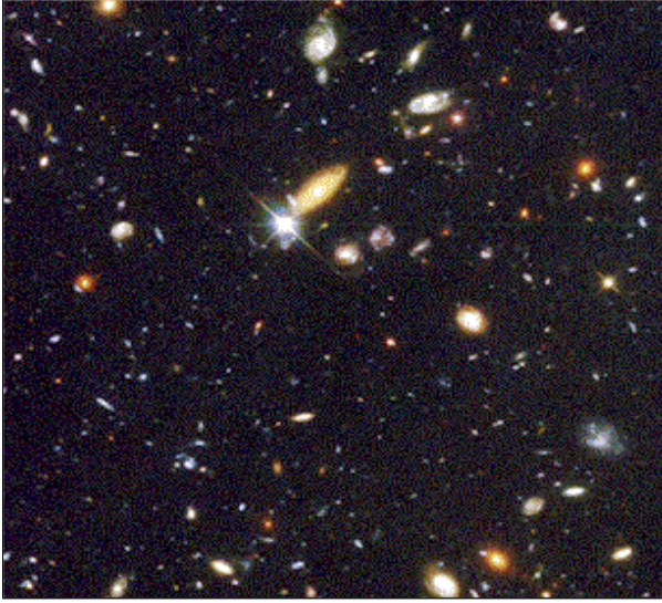
10,000 Galaxies
